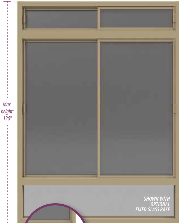
W3 Sliding window panel with transom and base Overall window panel heights including transom and base up to 120" Details about individual section parameters can be found under the pictures to the right.
